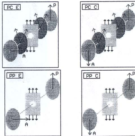
Figure 3. Polariscope arrangements.
