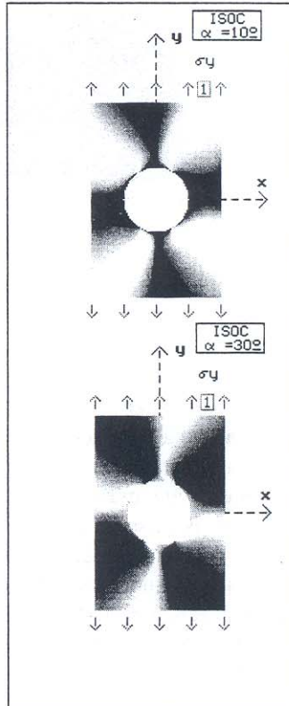
Figure 5. Examples of isolated isoclinics.
