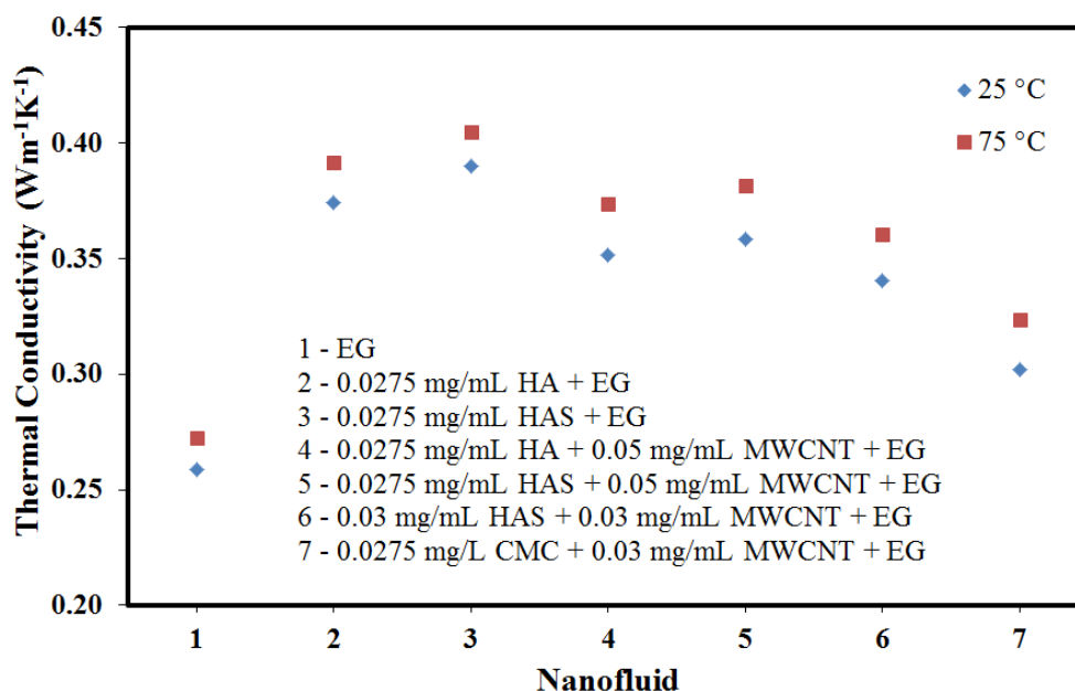
Figure 3. Thermal conductivity of the nanofluids.
