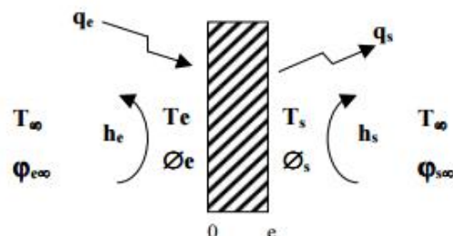
Figure 1. Heat transfer through a unidirectional plane wall.
