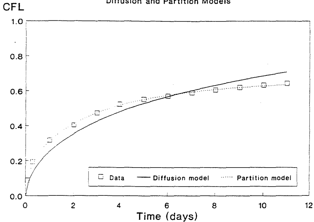
Figure A1. Experimental data as cumulative fraction leached, plotted as a function of time are shown as the squares. The finite cylinder diffusion model and the model in which the source term is partitioned are shown as lines fitted to the data. Data is for sodium leaching from portland cement containing sodium sulfate.
